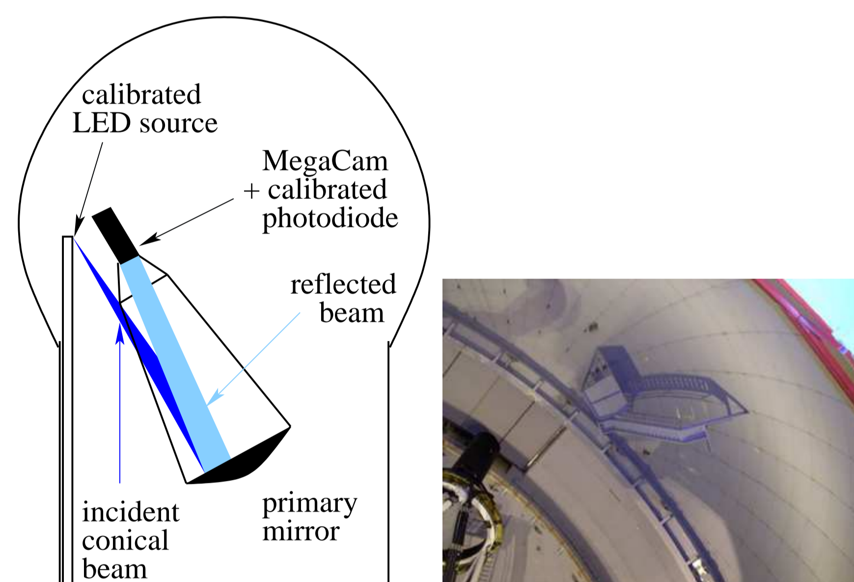
Figure 1: Inside the CFHT dome: the LED source will be attached to this platform.
