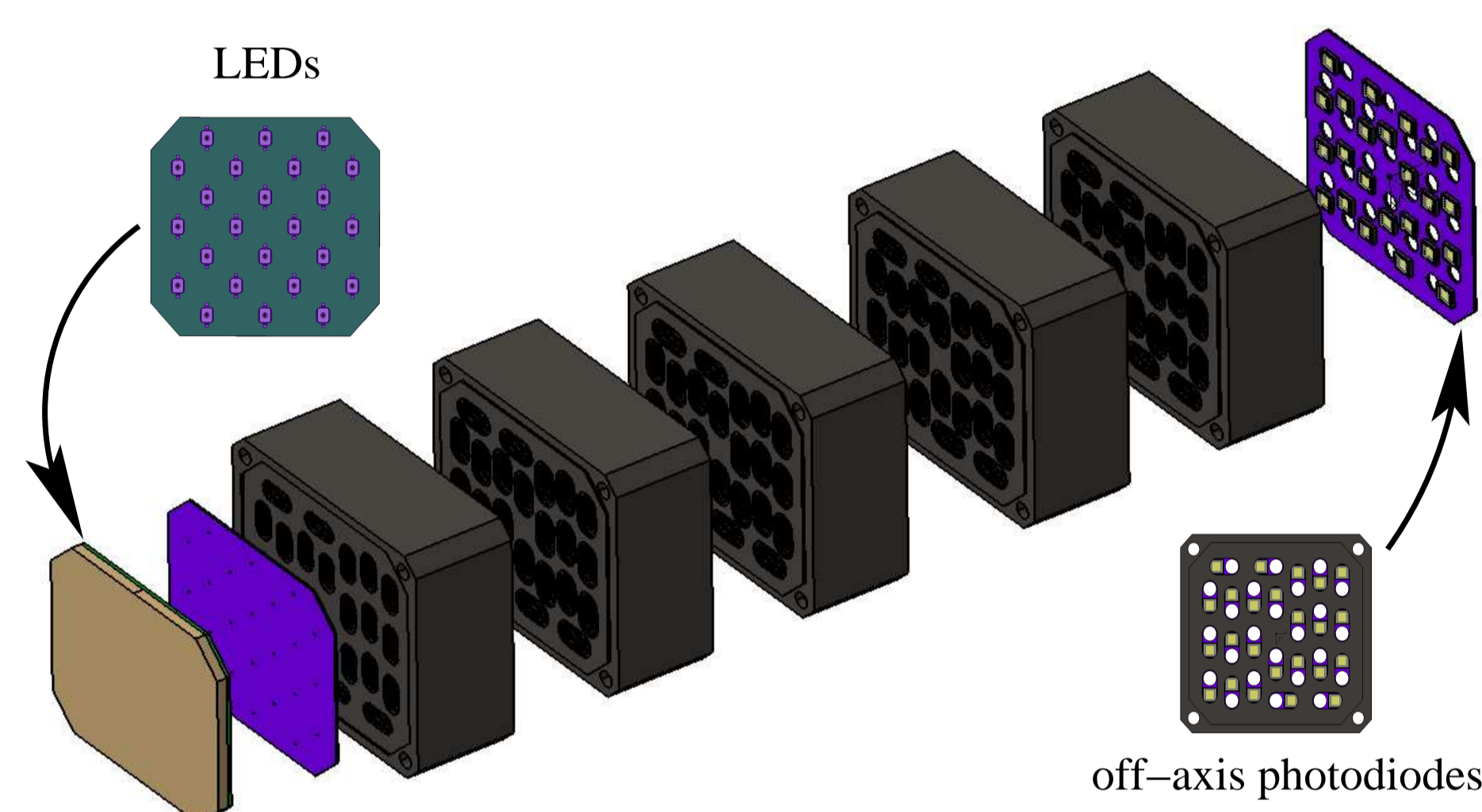
Figure 3: Design of the LEDs module with the LED plane, first mask, baffling and end mask with monitoring off-axis photodiodes.
