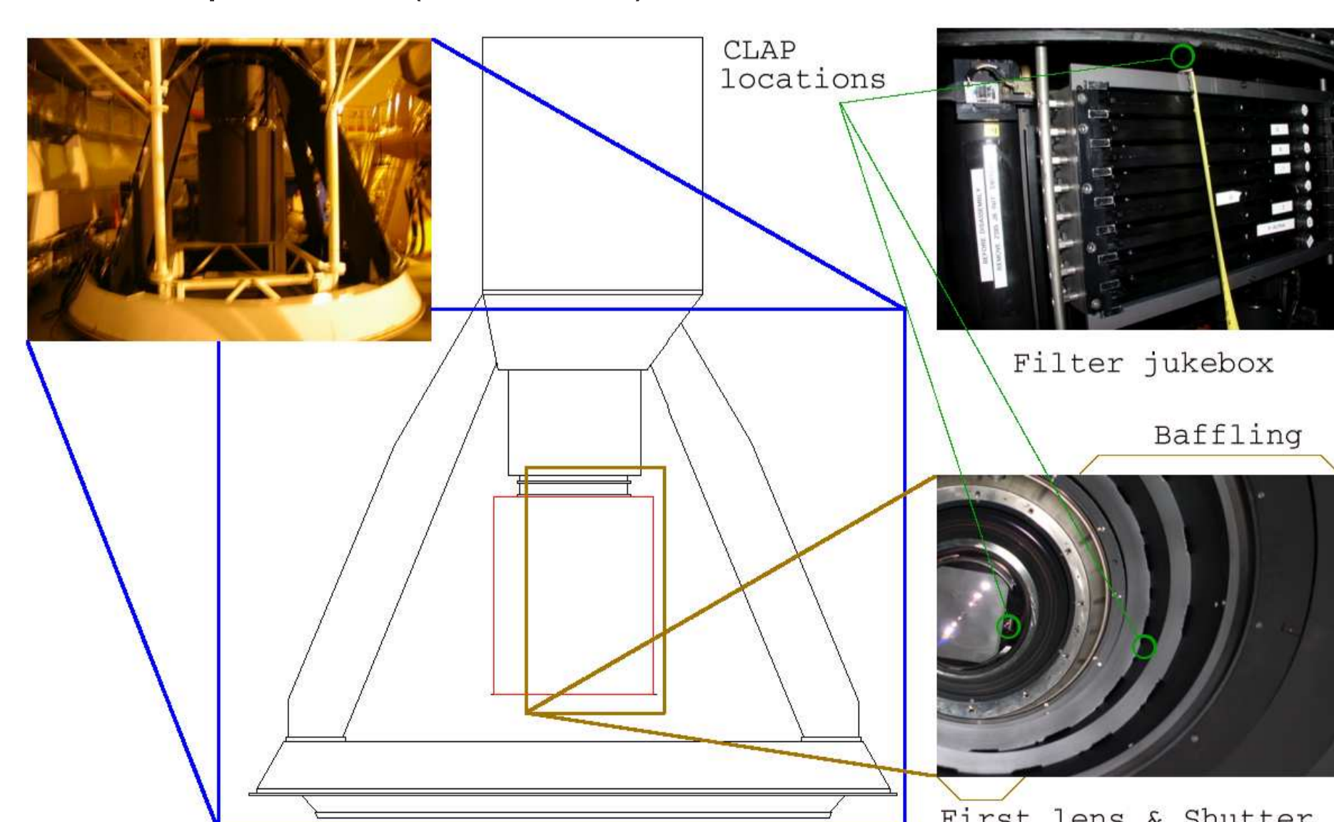
Figure 2: Three proposed positions for CLAPs: inside the baffling, behind the first lens using the same light path as the guiding (on the side of the shutter), and between the filter jukebox and the MegaCam cryostat, right next to the cryostat opening.
