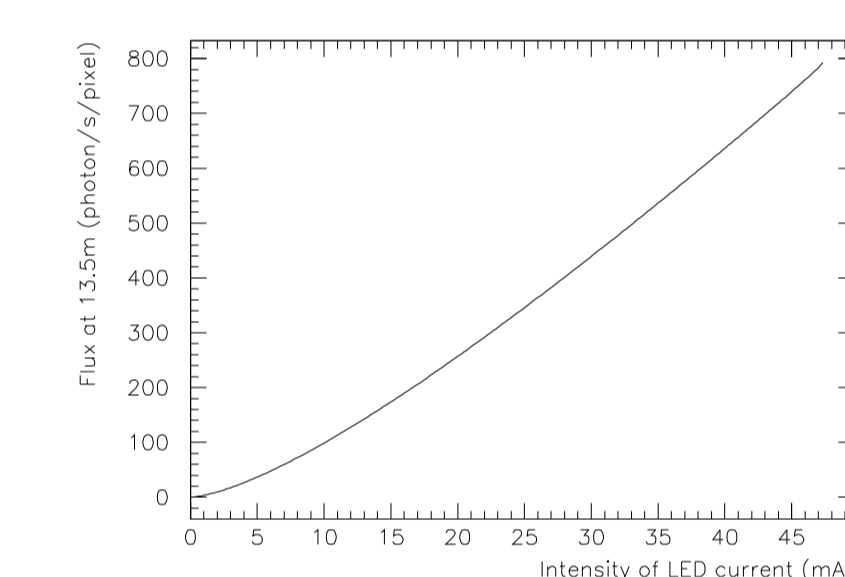
Figure 7: Flux in photons/s/pixel expected on MegaCam as a function of the current in a Golden Dragon LED (based on test bench measurements on a photodiode). The current in a Golden Dragon can go up to 300 mA, giving then 20,000 photon/s/pixel.
