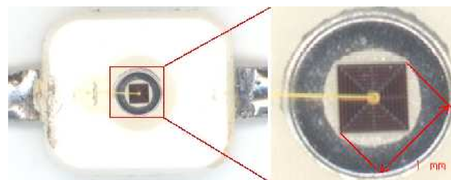
Figure 4: A Golden Dragon OSRAM LED, with a zoom on the photoemitting 'dice' (dark square, in center). The golden wire is one of the electrodes.
