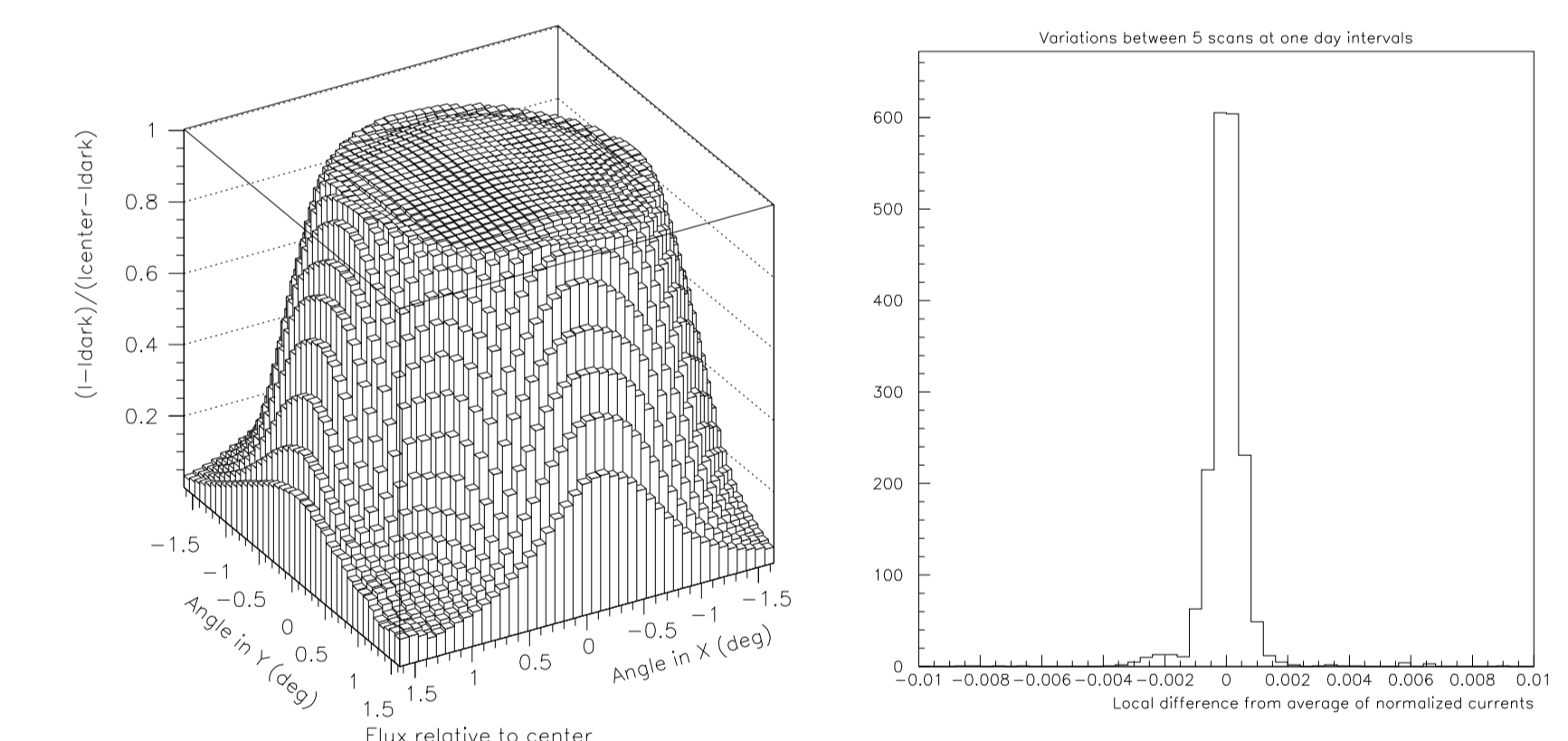
Figure 8: Map of the luminous field (relative to center) of an Agilent LED in the first prototype of LED source (left). Stability of the field map: local difference from average of five scans taken at one-day intervals (right).
