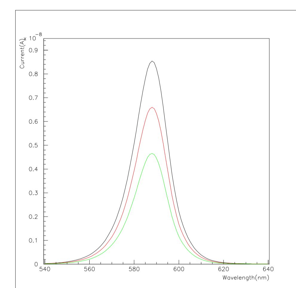
Figure 9: Spectrum of an orange Golden Dragon LED for three different LED currents.
