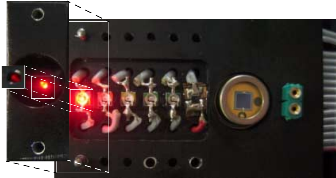
Figure 4 This light source model built at LPNHE/Paris is made of six LEDs on a base plate. The left most LED is lit. The same LED is also seen through a \text{Ø}0.5 mm hole drilled in a “low-mask” and through a \text{Ø}2 mm hole in a “high-mask”. Reflection on the edge of this thick hole yield a bump on beam profile (Figure 5). These three views are overlaid to suggest the mounting of the masks on the base plate. The photodiode seen on the right measures the light reflected on the optics and the detectors.
