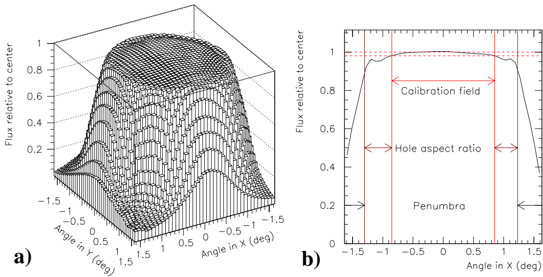
Figure 5 a) XY scan of the illumination field of the LED light source model shown in Figure 4. The photocurrent in the central flat field, generated by a 5.8 \text{ mm}^2 photodiode at 0.9 \text{ m} , is about 120 \text{ pA} b) a cut of this field along a symmetry axis shows a \pm 0.8^\circ calibration field with a \pm 1\% uniformity, surrounded by 0.4^\circ rougher region due to a bad aspect of the angular diaphragm and a penumbra zone
