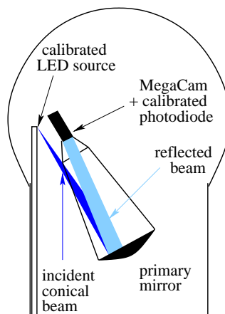
Figure 3 Dome setup for the SNLS experiment: the CLED source is at a fixed position inside the dome, the telescope is pointed towards the source for calibration exposure.
