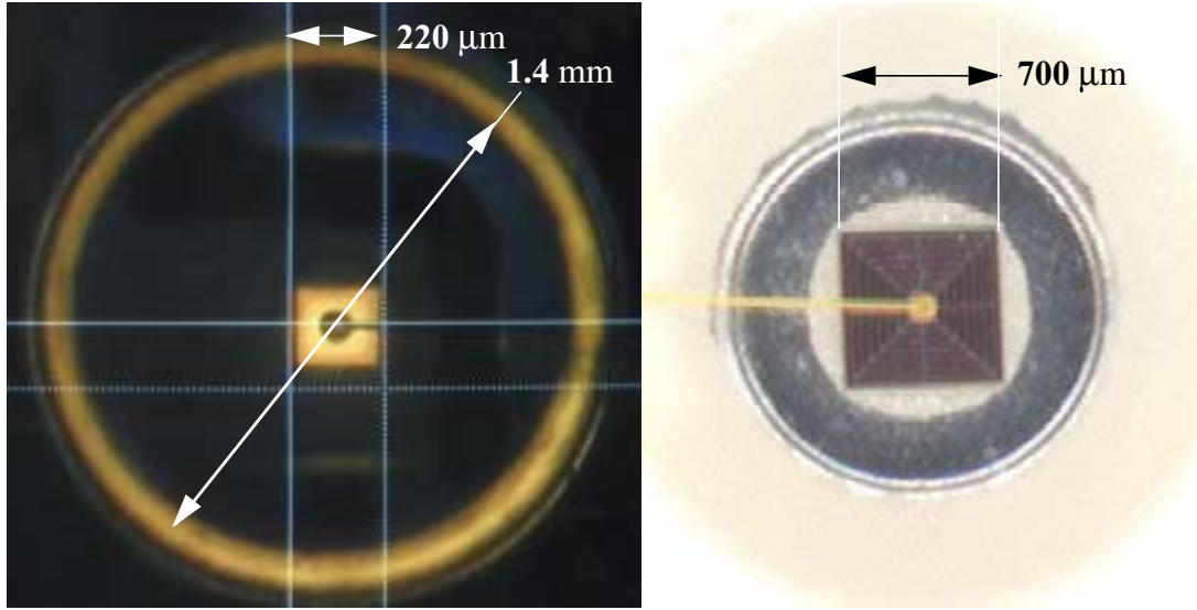
Figure 1 Flat-top LEDs: Left Agilent “P505” - Right Osram “golden dragon” (respective quantum efficiencies 0.1% and 5% cf. Appendix B). Light emission is confined to central squares (0.2x0.2 and 0.7x0.7 mm). Light ring around P505 (Ø1.4mm) is coming from diffusion on the cylindrical plastic wall. It has to be masked (see Figure 4).
