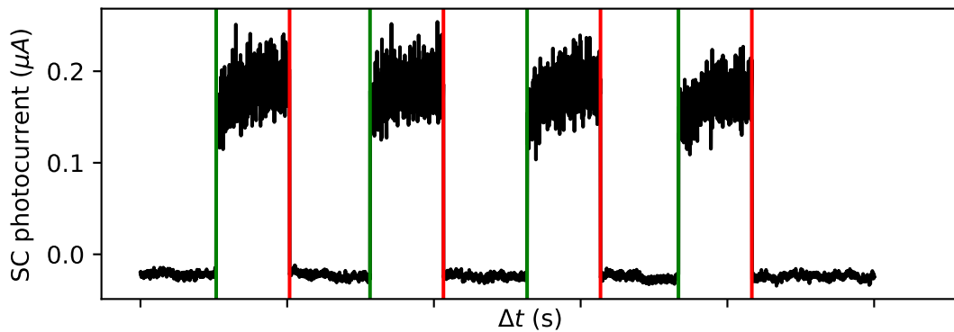
Data for \lambda = 598
