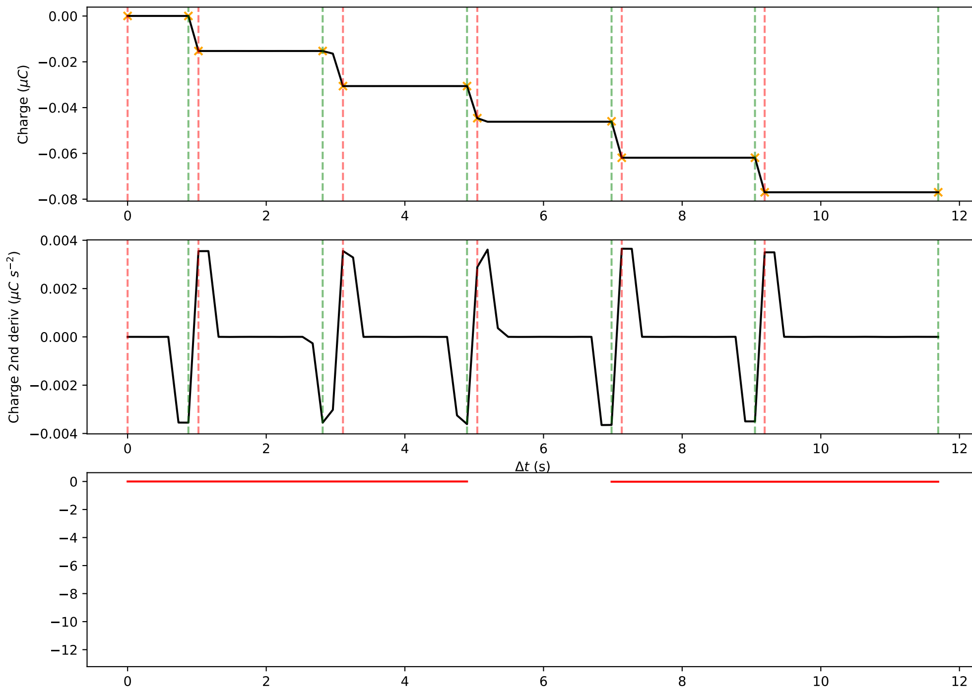
PD data for \lambda = 975\text{nm}
