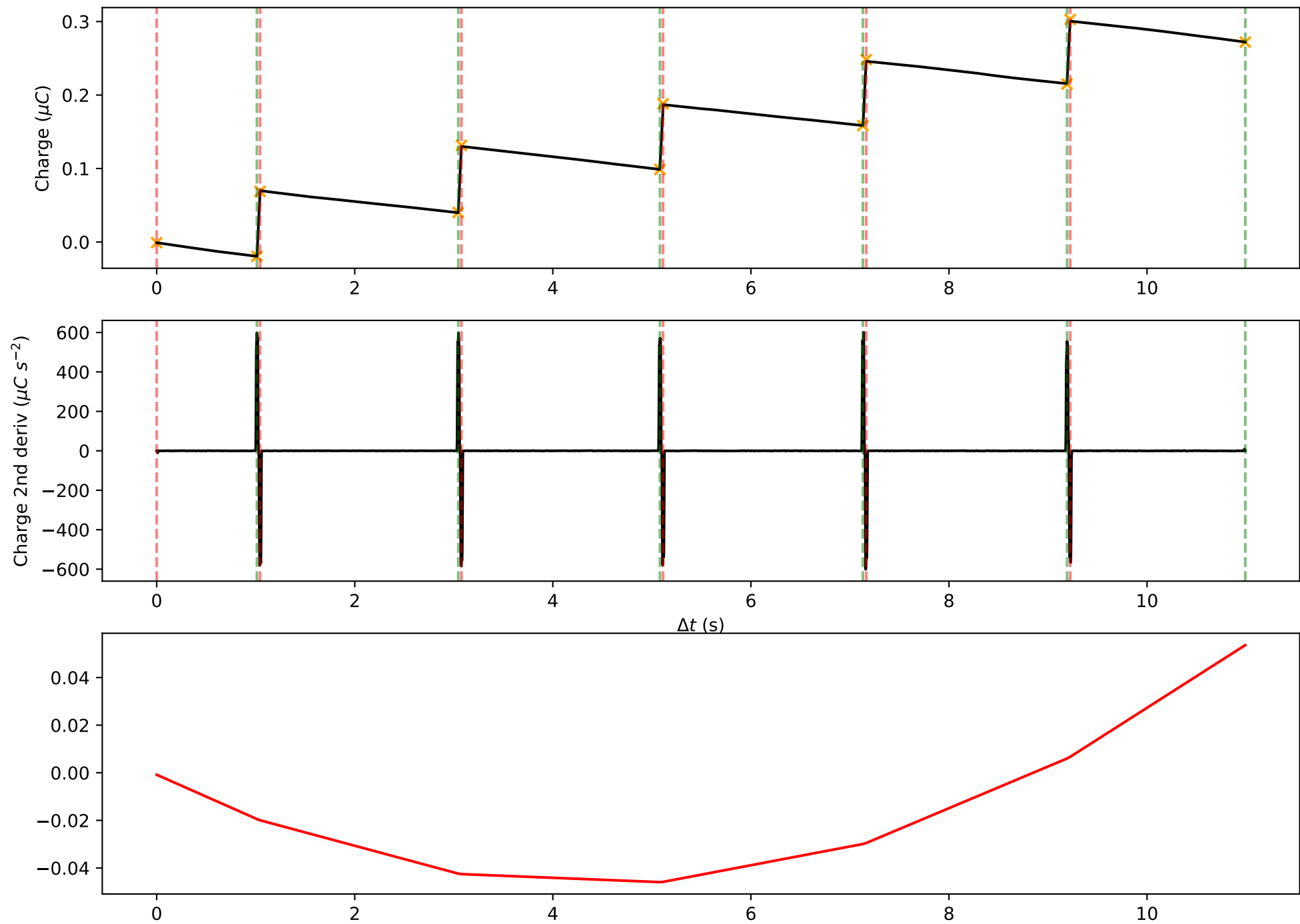
SC data for \lambda = 1005\text{nm}
