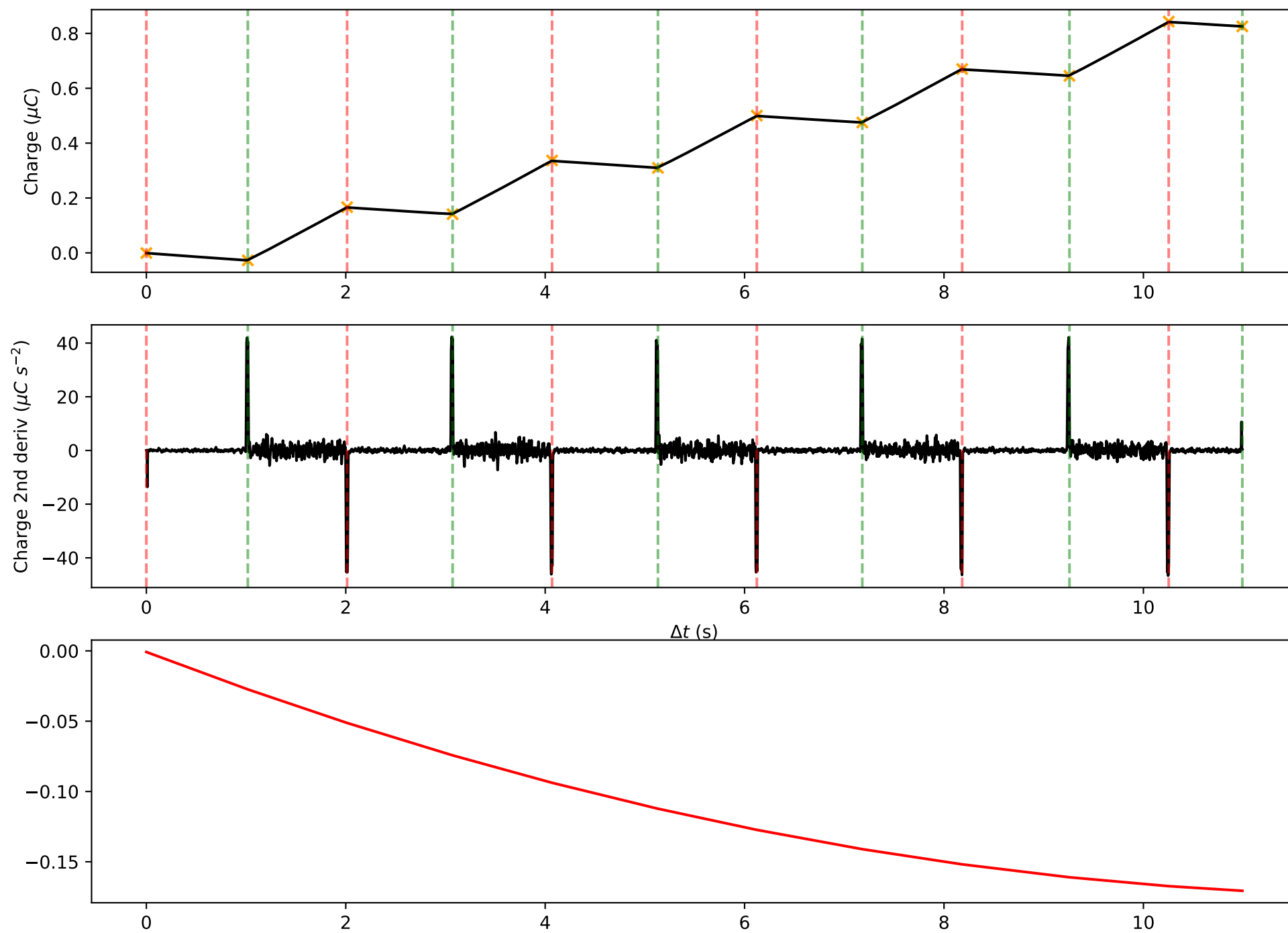
SC data for \lambda = 370\text{nm}
