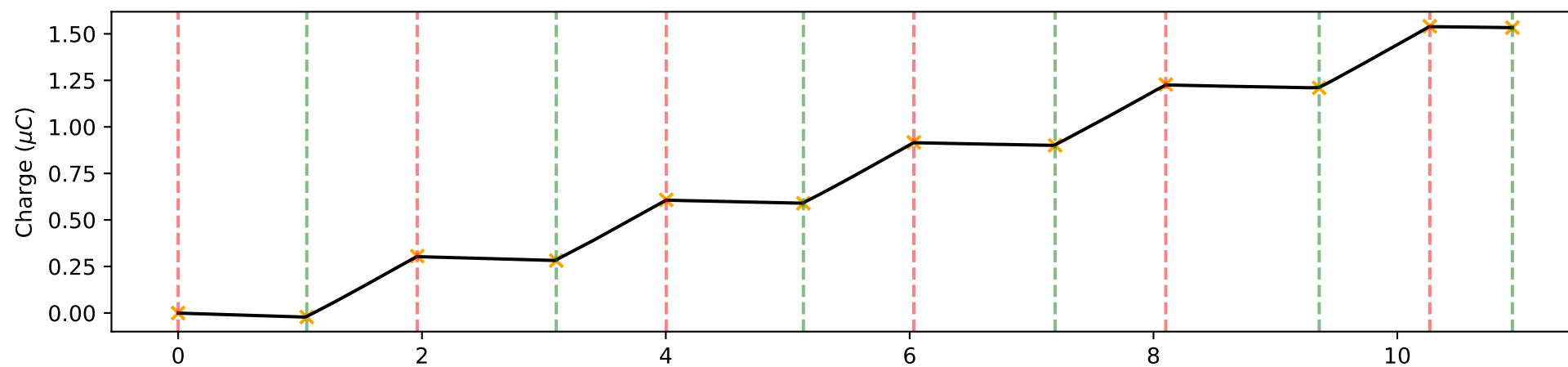
SC data for \lambda = 420\text{nm}
