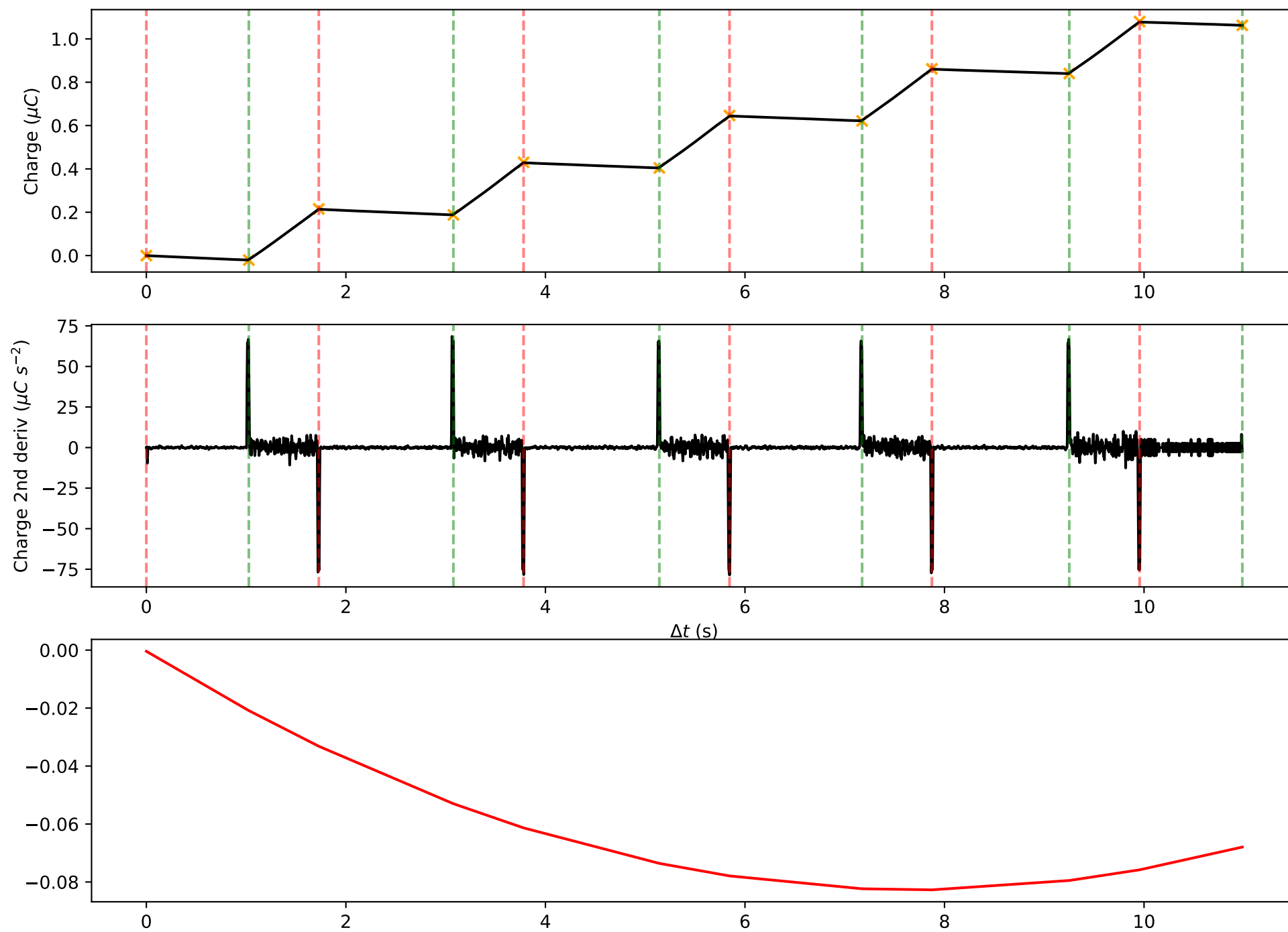
SC data for \lambda = 455\text{nm}
