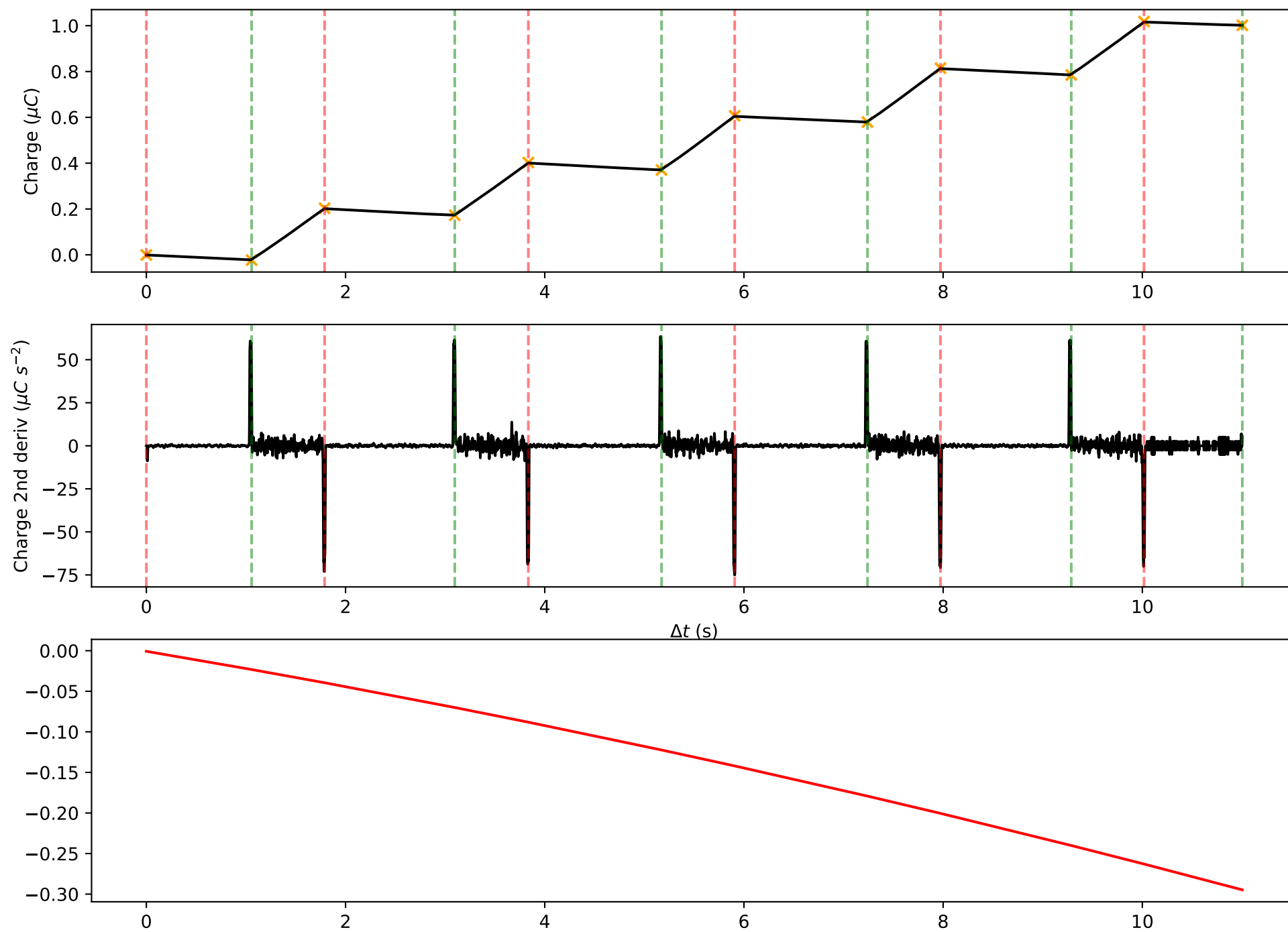
SC data for \lambda = 465\text{nm}
