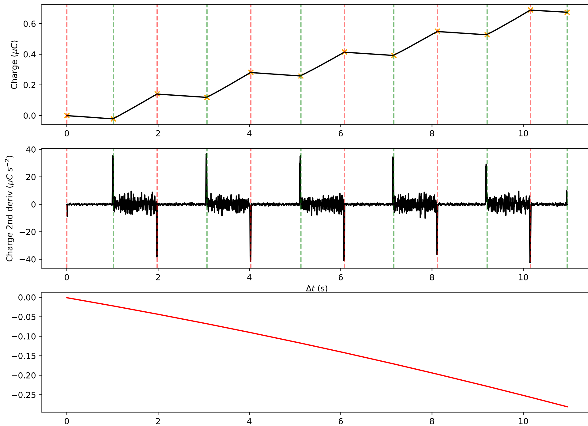
SC data for \lambda = 545\text{nm}
