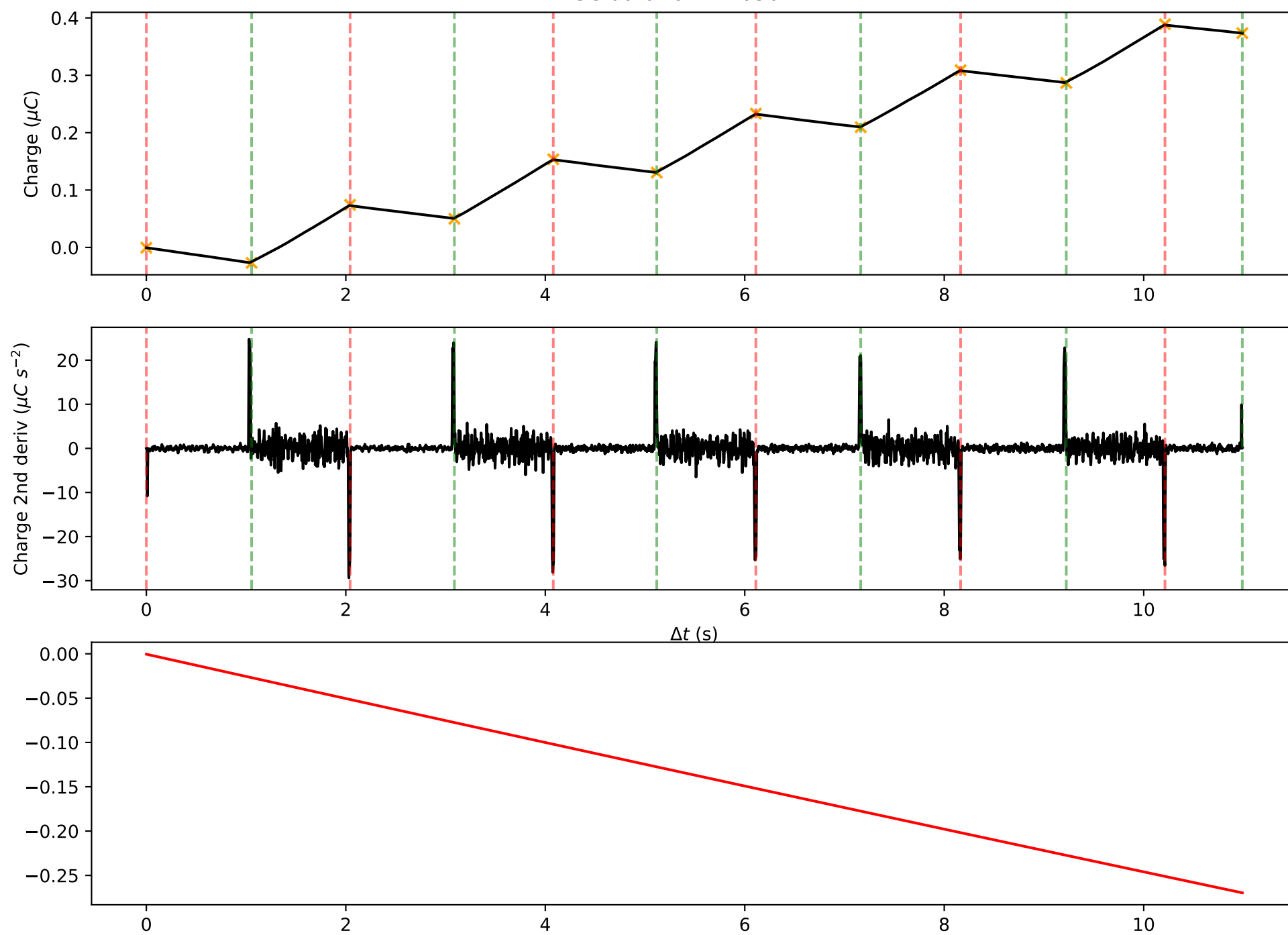
SC data for \lambda = 630\text{nm}
