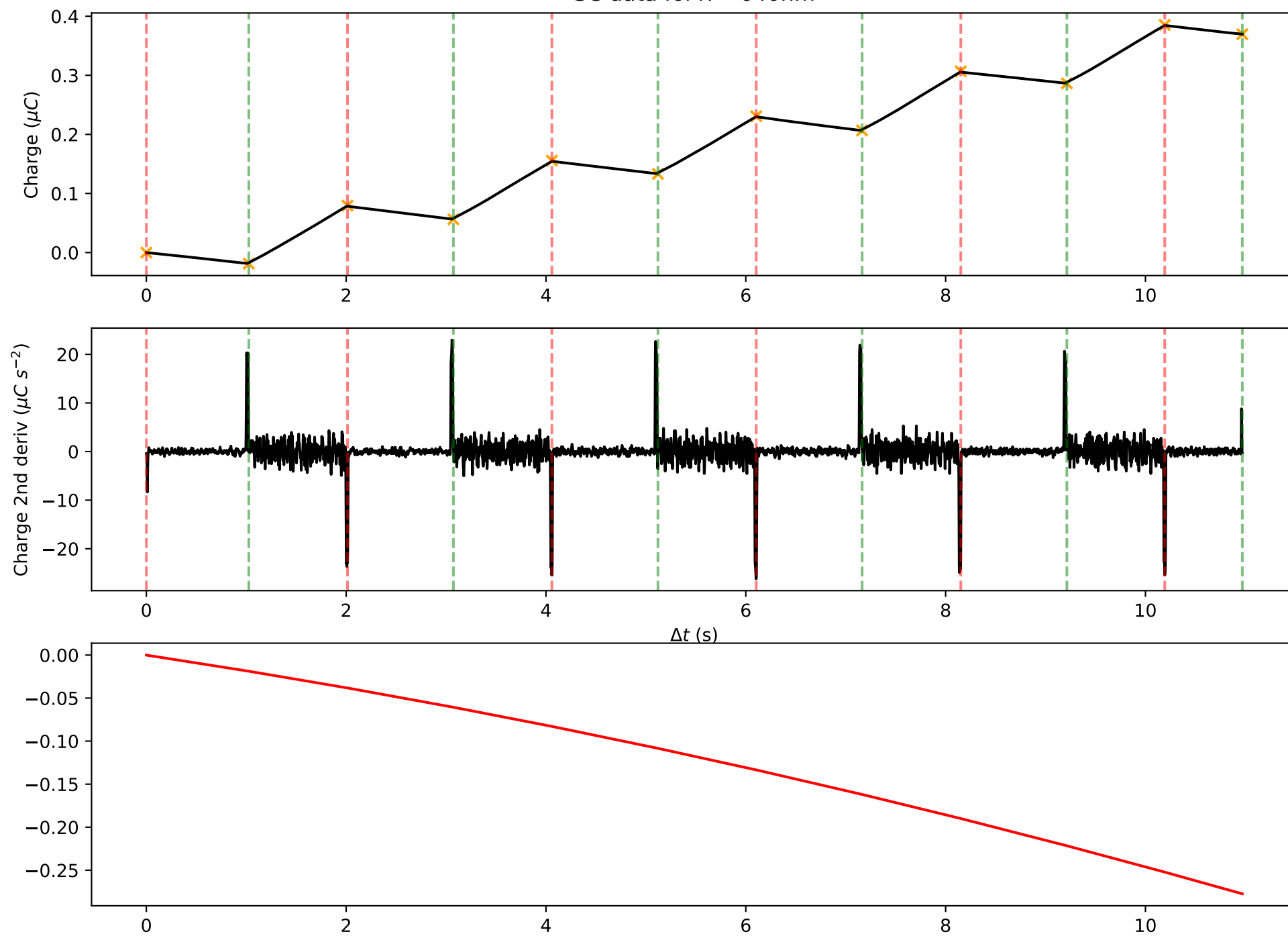
SC data for \lambda = 640\text{nm}
