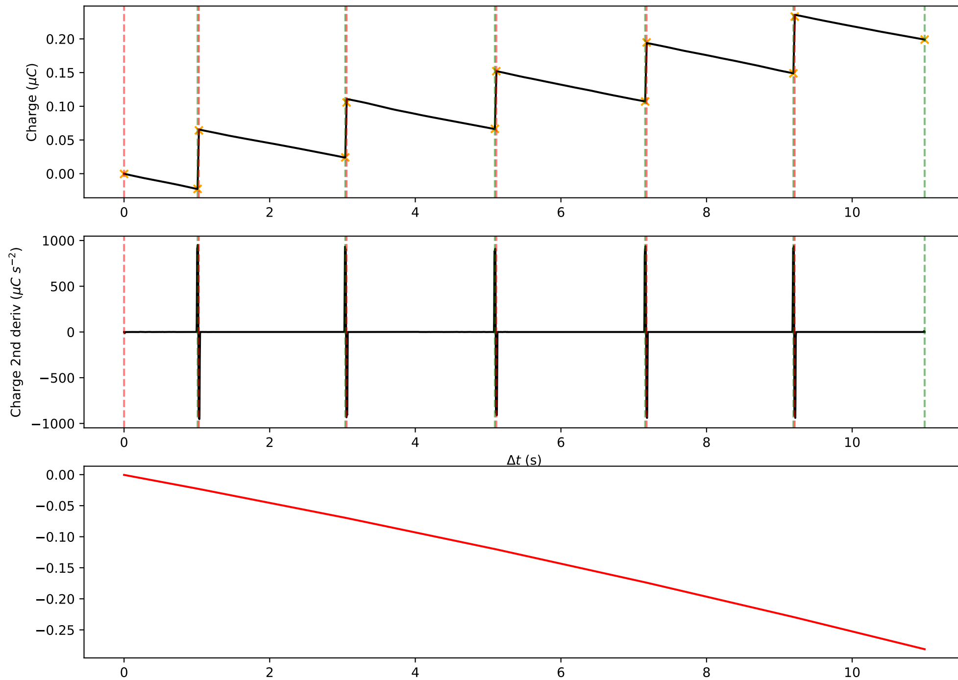
SC data for \lambda = 745\text{nm}
