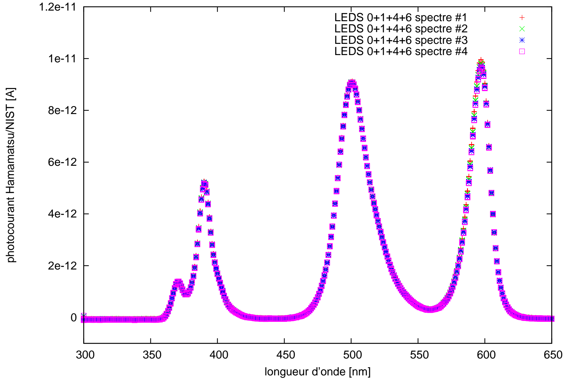
Spectres des LEDs 0, 1, 4 et 6 (grating 3)
