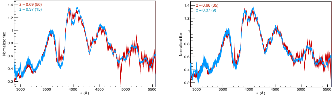
Figure 2: Mean spectra at low (in blue) and high (in red) redshift built from the VLT sample with 15 low z and 56 high z spectra (left) and from two VLT sub-samples with similar photometric properties in average with 9 low z and 35 high z spectra (right)
