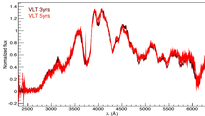
Figure 1: Mean spectra from VLT 3 year (in dark red) and VLT 5 year (in light red) samples
