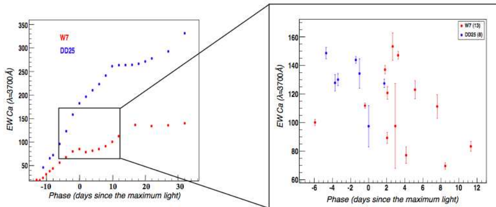
Fig. 4. Time evolution of EW Ca Left: for W7 (red) and DD25 (blue) model spectra Right: Same as left for the two observed spectra subsamples best fitted by W7 (red) and DD25 (blue). The ranges of EW Ca values and phases match those shown in the box on the left panel
