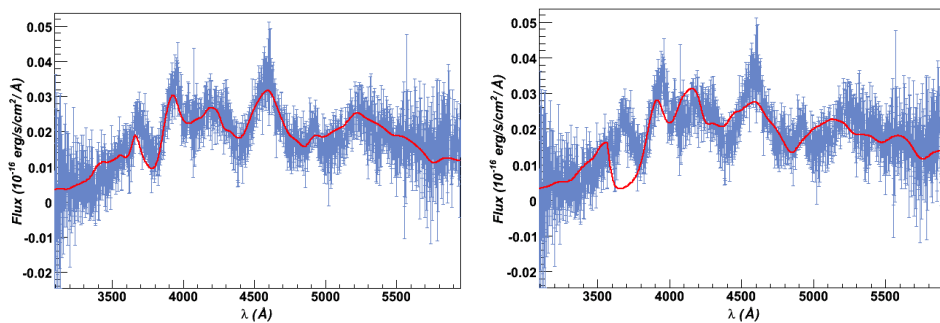
Fig. 2. SN 04D2cf (blue) at z=0.368 with phase=8.48 days, fitted by the models (red) Left: 24 days W7 spectrum (best fit) Right: 20 days DD25 spectrum
