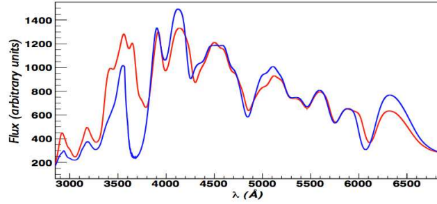
Fig. 1. Overlap of 18 days W7 (red line) and 18 days DD25 (blue line) spectra showing the spectral differences between the models
