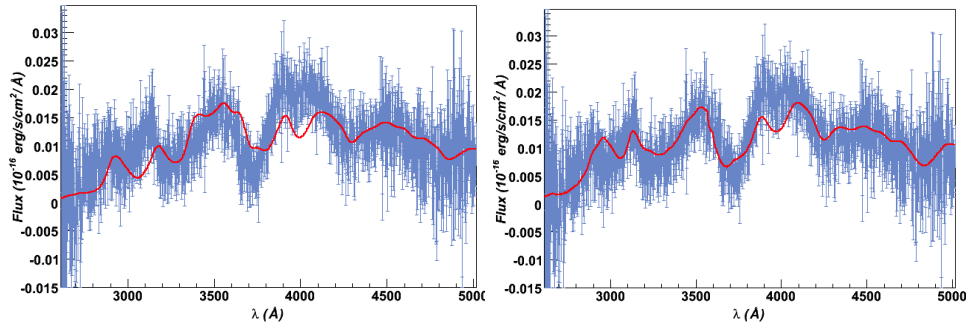
Fig. 3. SN 04D2an (blue) at z=0.362 with phase= -3.39 days, fitted by the models (red) Left: 16 days W7 spectrum Right: 14 days DD25 spectrum (best fit)
