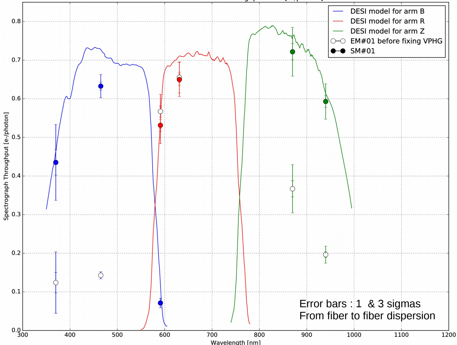
Direct estimate of the throughput ratio [e-/photon]
