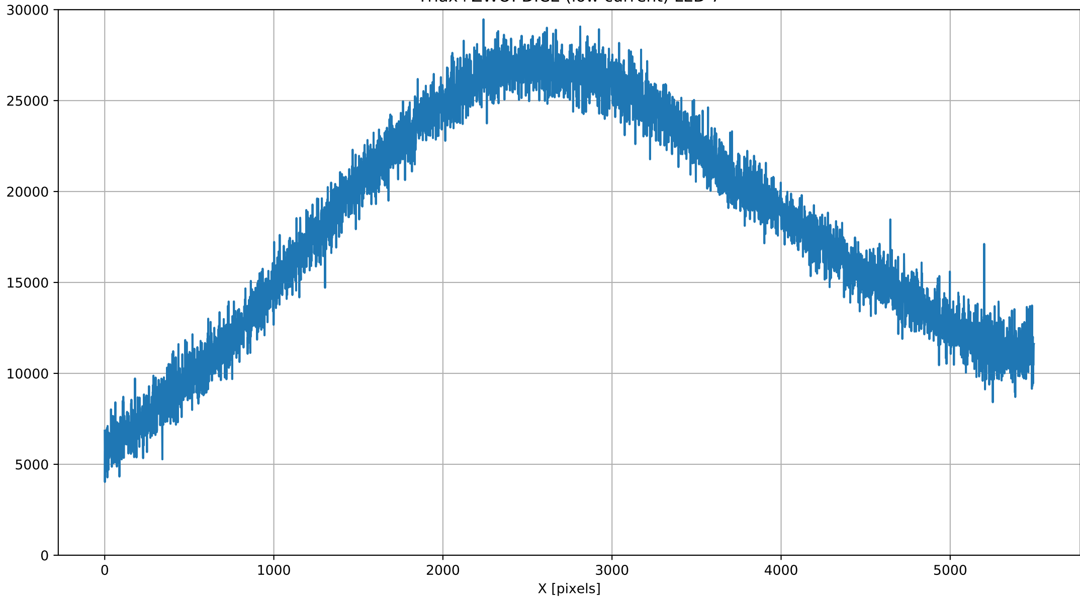
Triax+ZWO: DICE (low current) LED 7
