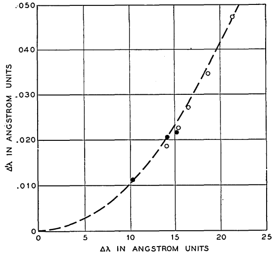
FIG. 14. Computed and observed second-order shifts, plotted against first-order (Doppler) shifts.
