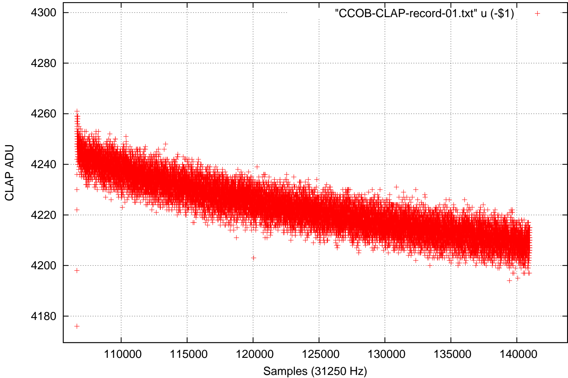
CCOB pulses as recorded by the LPNHE CLAP
