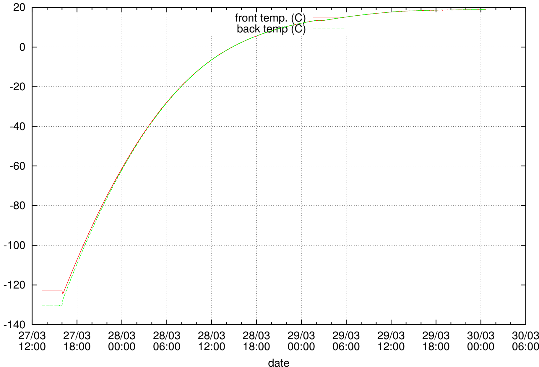
dewar temperature
