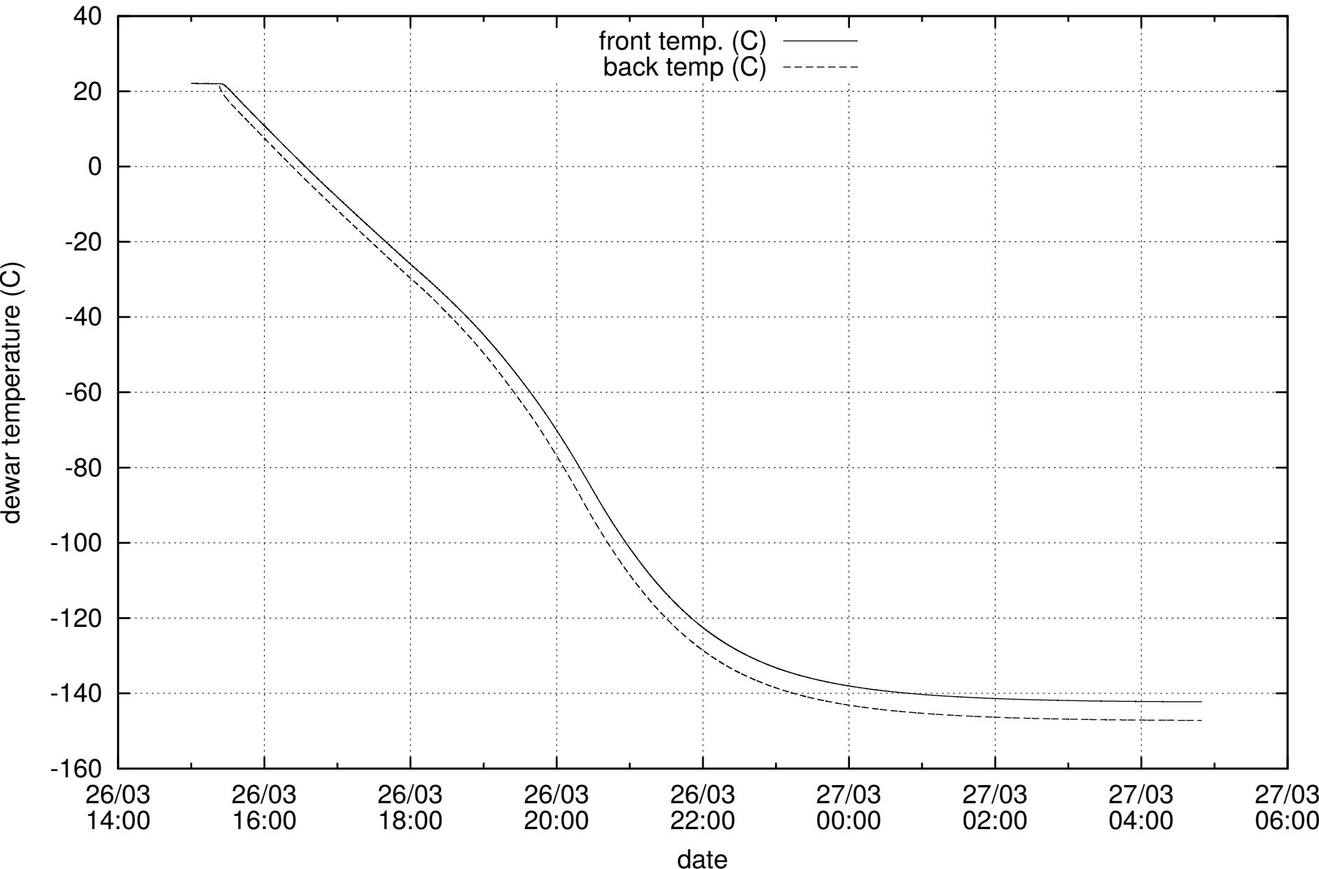
dewar temperature
