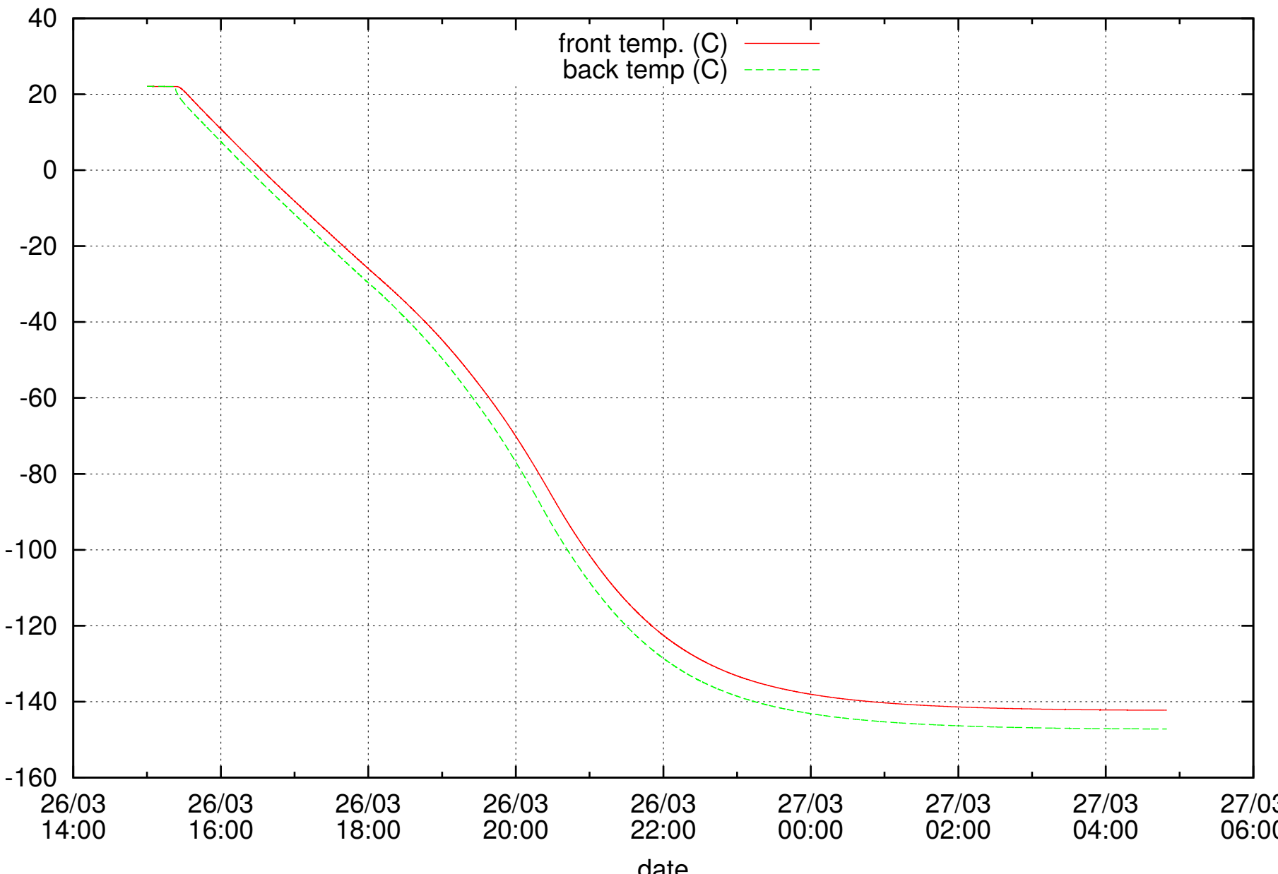
dewar temperature
